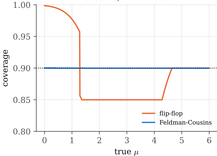
Gaussian, nominal 90%
