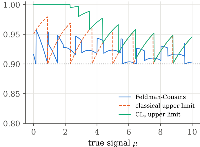
Poisson, b = 3 , nominal 90%
