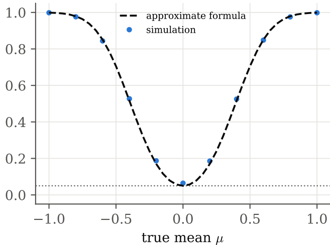
two-sided Wald, n = 25
