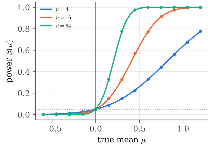
one-sided, H_0 : \mu \leq 0
