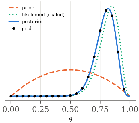
Beta(2,2) + 17 of 20 heads
