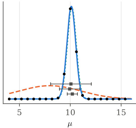
Normal(8,3) + three measurements
