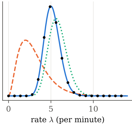
Gamma(3,1) + counts 3, 5, 7, 4, 9
