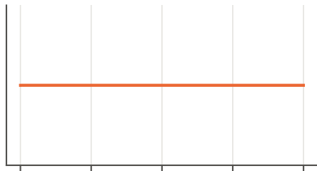
prior Beta(1, 1)
