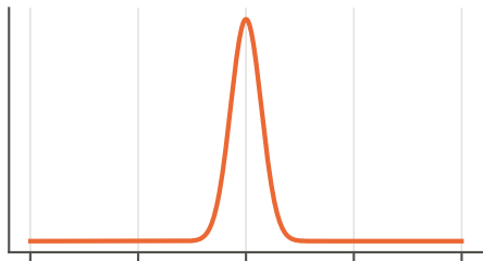
prior Beta(100, 100)
