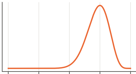
prior Beta(18.25, 6.75)
