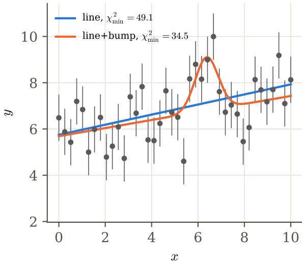
data with a bump: \ln B_{10} = 2.1
