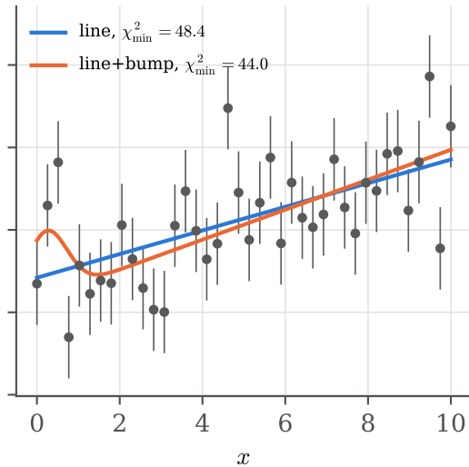
data without a bump: \ln B_{10} = -1.7
