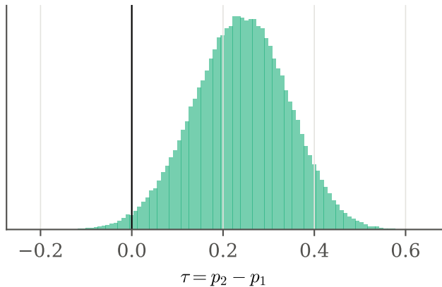
a difference, by subtracting draws
