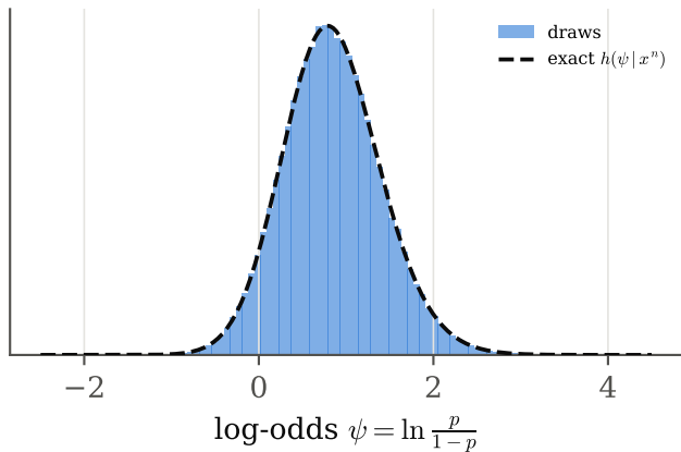
a difference, by subtracting draws
