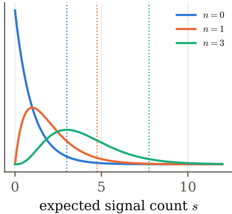
collider: counts
