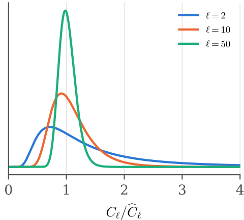
CMB: band power
