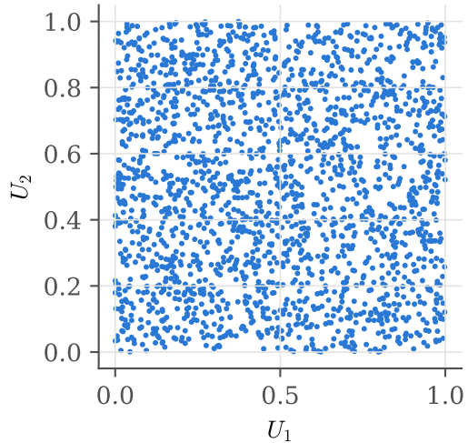
uniform input
