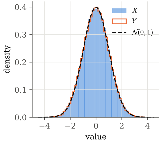
histograms
