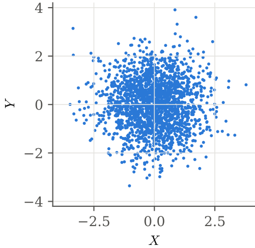
Gaussian output
