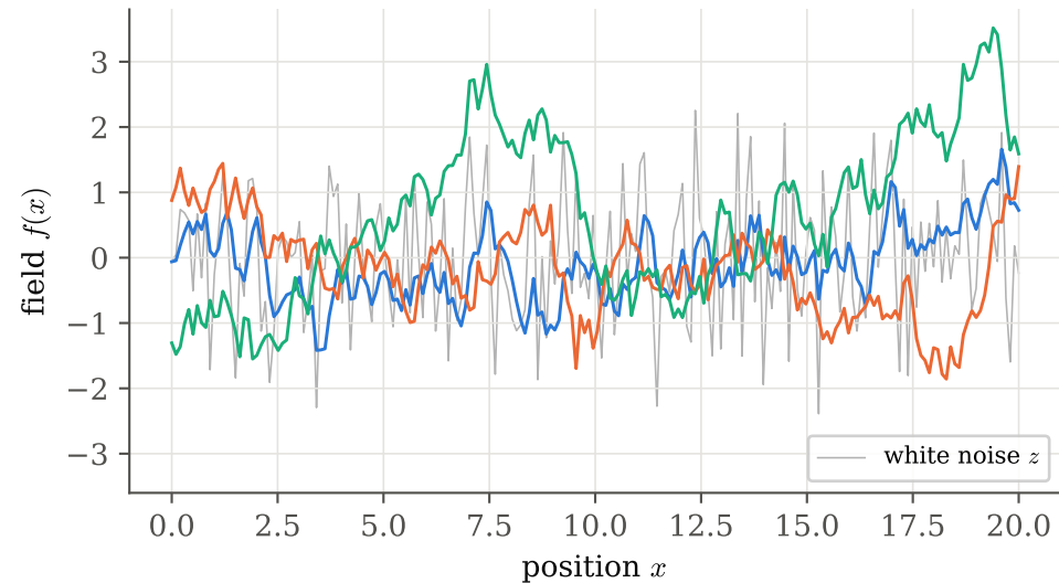
realisations of f = \mathbf{L}z
