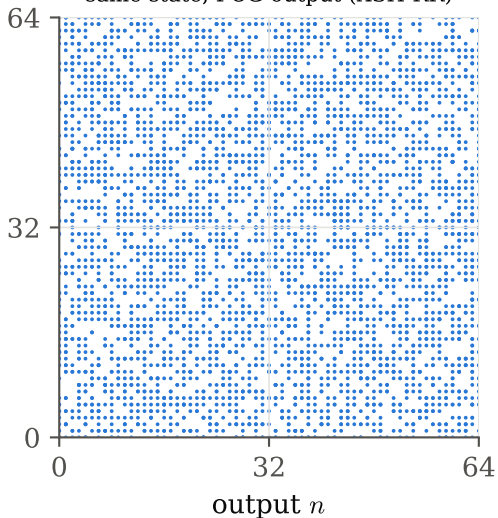
same state, PCG output (XSH-RR)
