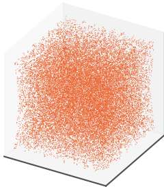
RANDU, generic view
