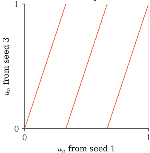
RANDU: seed 1 against seed 3
