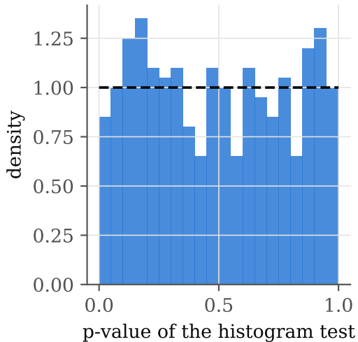
PCG64, 400 batches of 10^4
