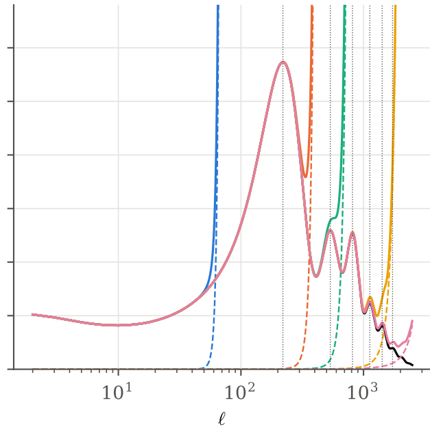
deconvolved: D_\ell + \text{noise } N_\ell/B_\ell^2 (dashed), 30 \mu\text{K}'
