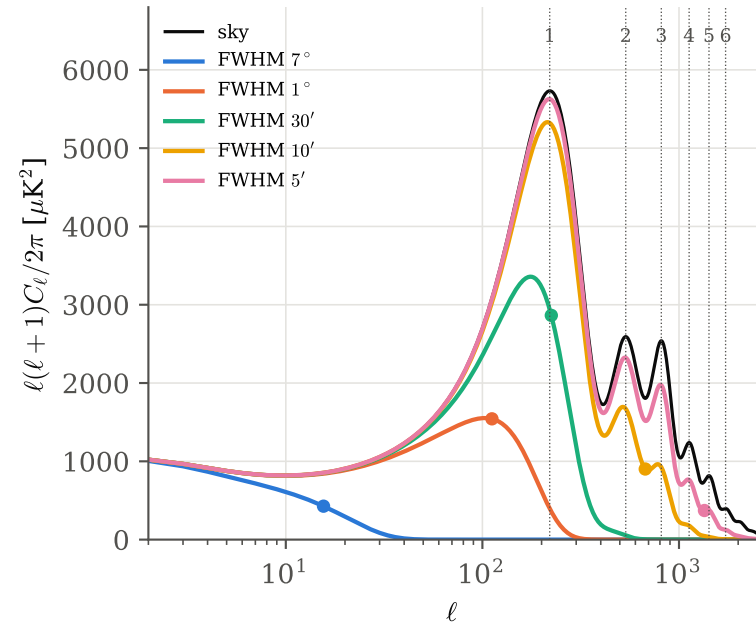
observed: D_\ell B_\ell^2 (dots: B_\ell^2 = 1/2 )
