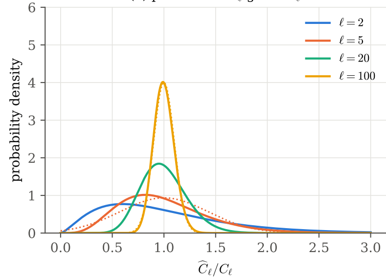
(a) prediction: \widehat{C}_\ell given C_\ell
