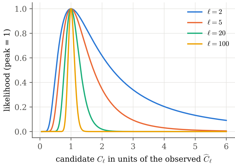
(b) inference: which C_\ell made our \widehat{C}_\ell ?
