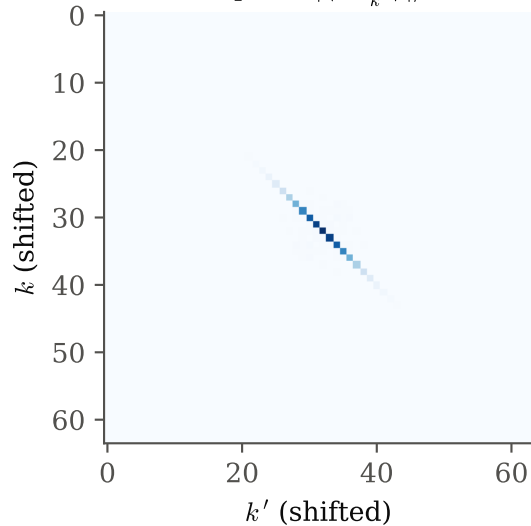
Fourier space: |\langle \delta_k \delta_{k'}^* \rangle|/n (sim.)
