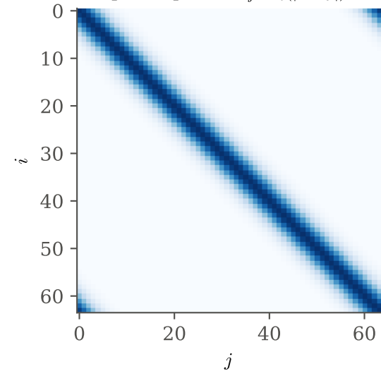
pixel space: C_{ij} = \xi(|i - j|)
