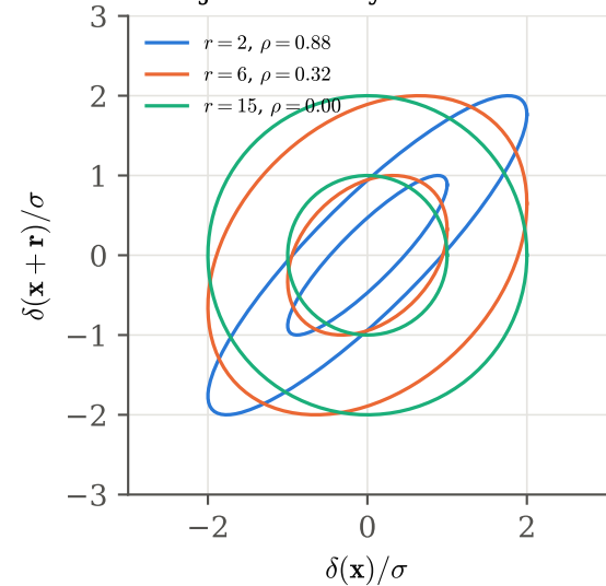
joint density: contours
