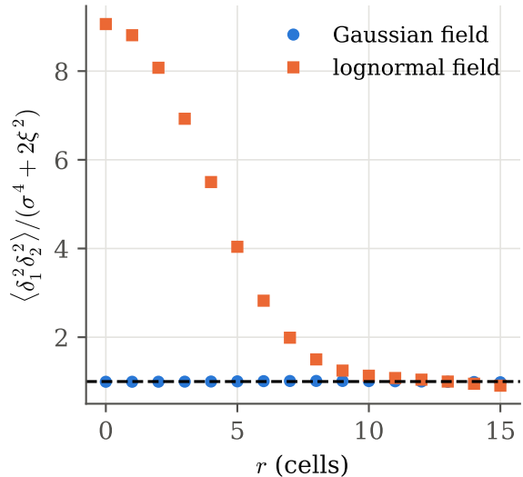
Wick test
