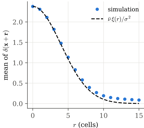
around pixels with \delta > 2\sigma
