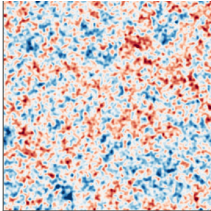
(c) |\delta_k| of rings, phases of blobs
