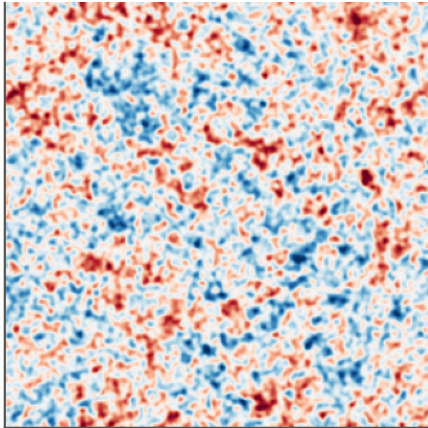
(b) same |\delta_k| , random phases
