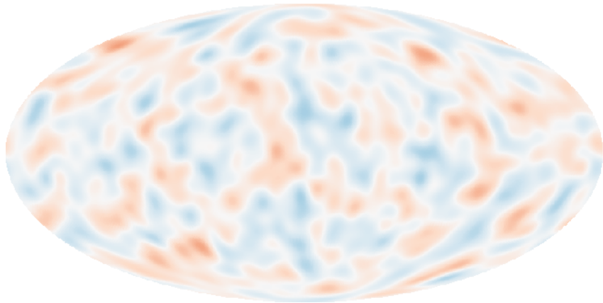
(b) same |a_{\ell m}| , random phases
