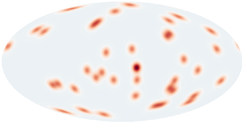
(a) 40 hot spots
