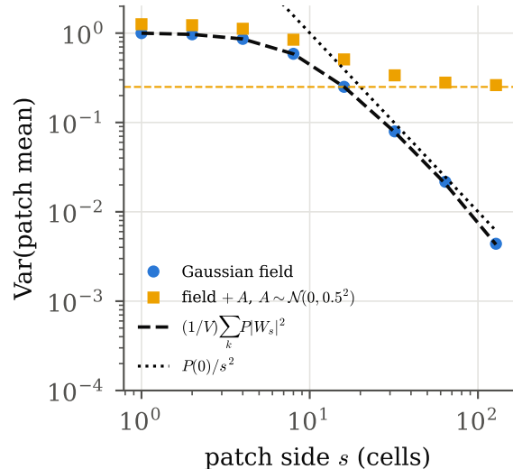
(c) spatial average
