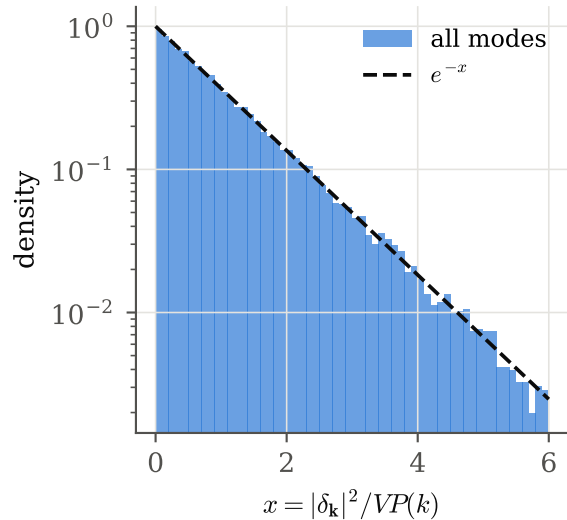
(a) power in one mode
