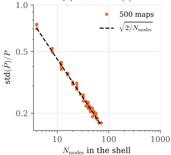
(b) scatter of \hat{P}(k)
