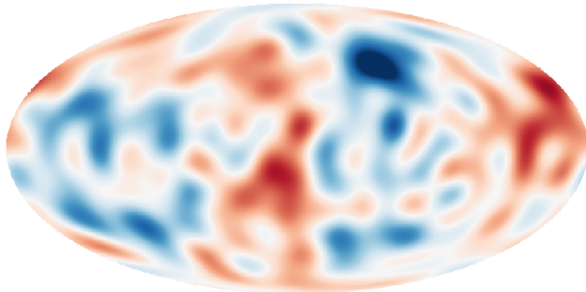
\ell \leq 600 (scale \pm 301 \mu\text{K} )
