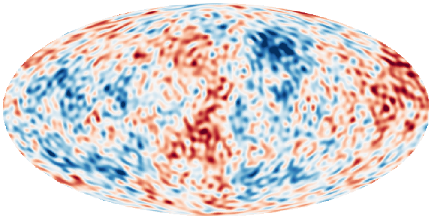
\ell \leq 64 (scale \pm 179 \mu\text{K} )
