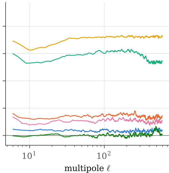
(b) r(\ell, \ell + 2)
