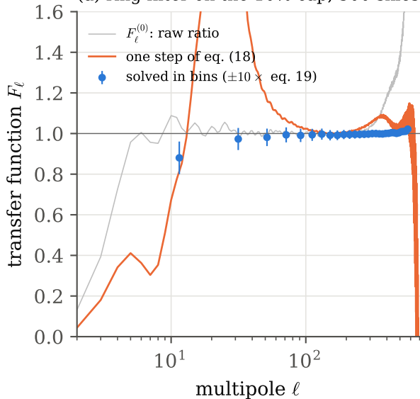
(a) ring filter on the 10% cap, 500 skies
