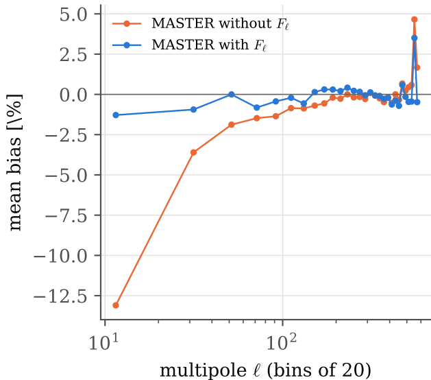
(b) 1500 independent test skies
