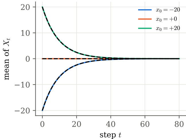
(a) the mean forgets x_0 as \rho^t x_0
