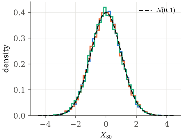
(b) all three starts end in the same law
