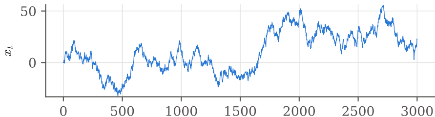
(b) accept with \min(1, f(y)/f(x)) : Metropolis (acceptance 0.54)
