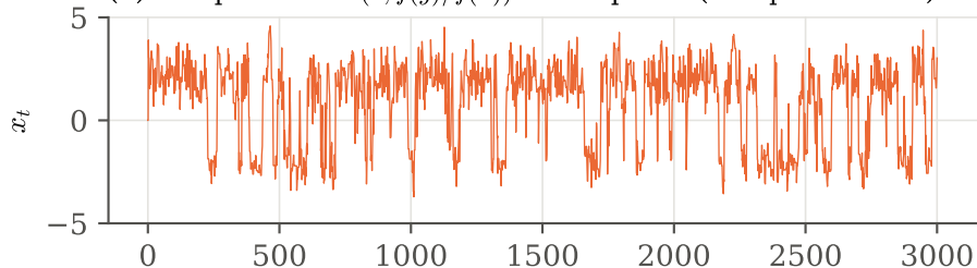
(c) accept only uphill: the hill climber (acceptance 0.00)
