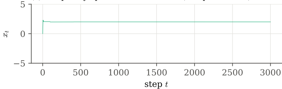
(c) accept only uphill: the hill climber (acceptance 0.00)
