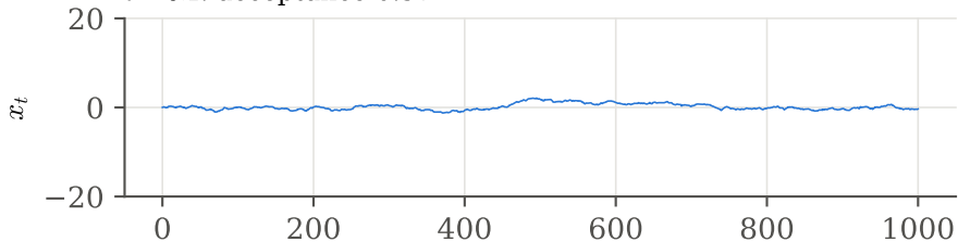
b = 1 : acceptance 0.84
