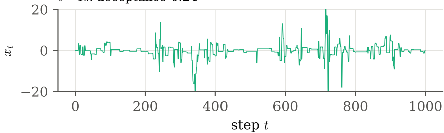
b = 10 : acceptance 0.24
