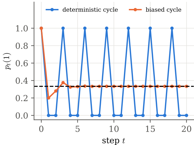
(a) probability of state 1
