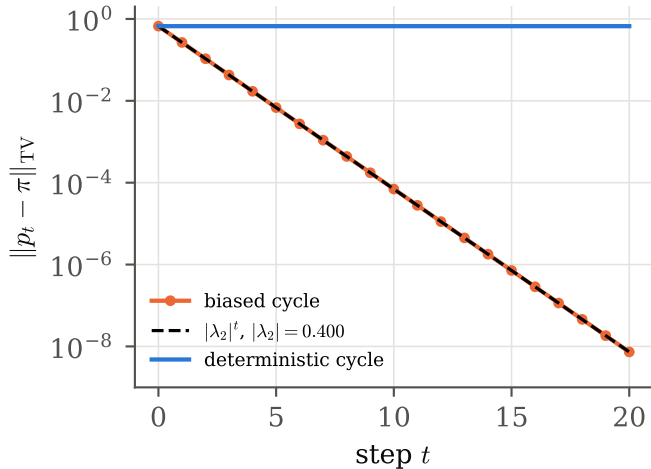
(b) distance to the uniform \pi
