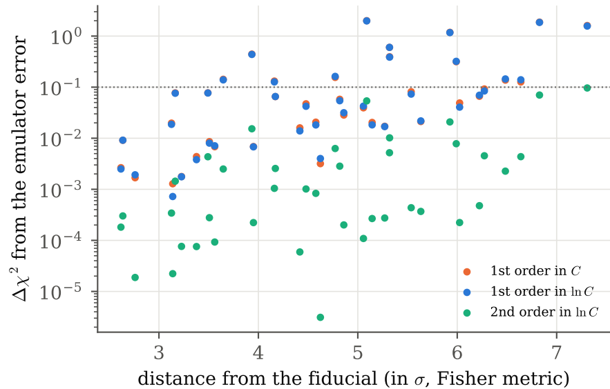
(b) 40 random models vs CAMB
