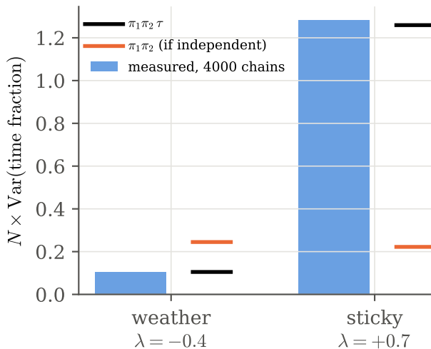
(a) two-state chains, N = 1000
