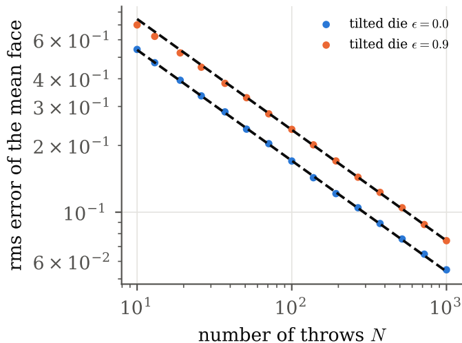
(b) error \sigma\sqrt{\tau/N} (dashed)
