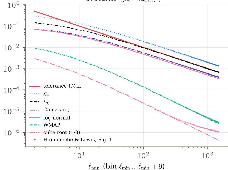
(b) scatter \langle (A_i - A_{\text{exact}})^2 \rangle^{1/2}
