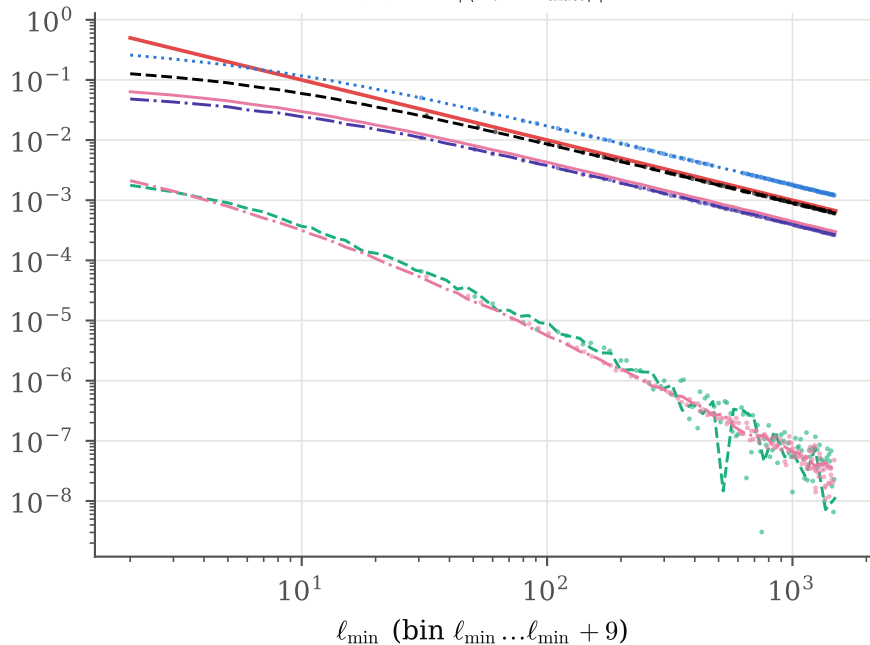
(a) bias |\langle A_i - A_{\text{exact}} \rangle|
