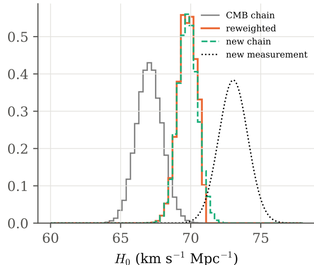
(c) in tension: ESS 634 of 144000
