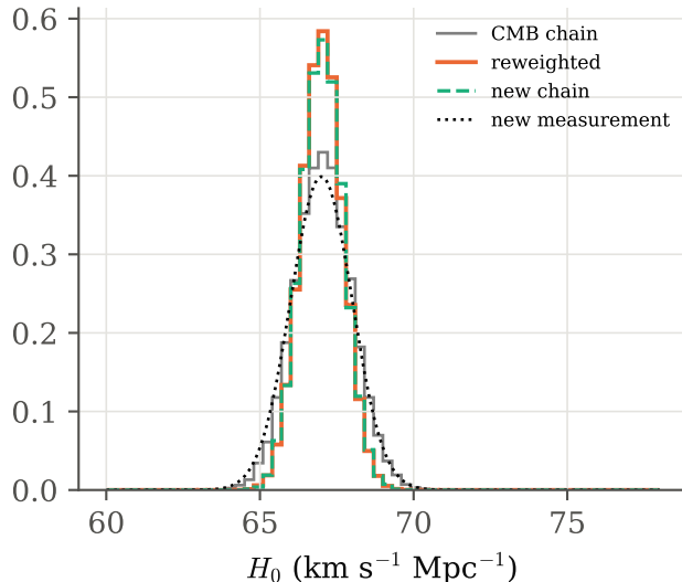
(b) compatible: ESS 127474 of 144000
