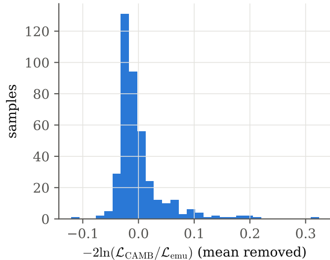
(a) 400 samples recomputed with CAMB
