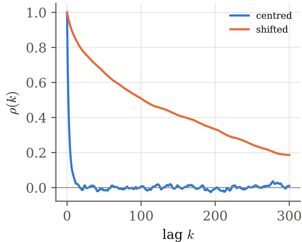
(b) autocorrelation of b
