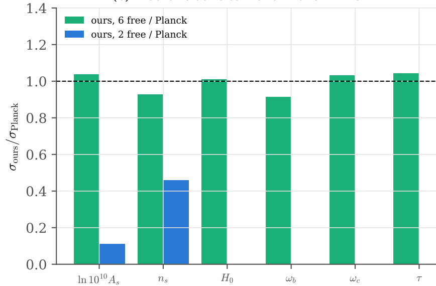
(b) widths relative to Planck 2018 TT+lowE
