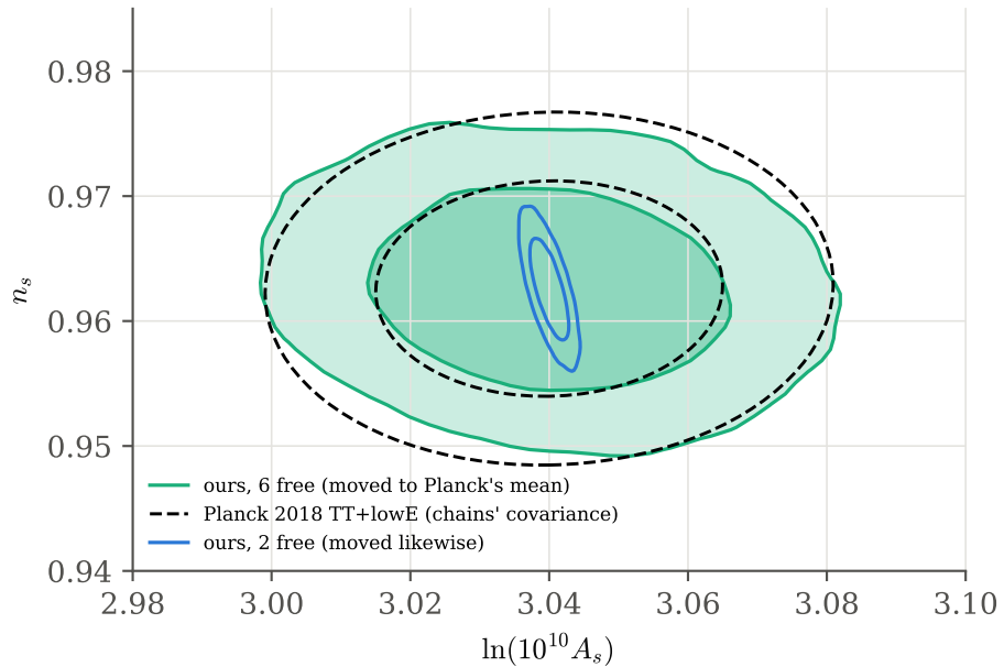
(a) (\ln A_s, n_s) : ours vs Planck
