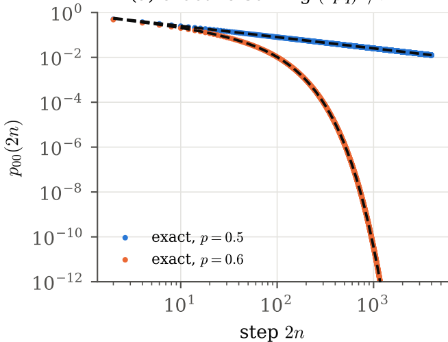
(a) exact vs Stirling (4pq)^n / \sqrt{\pi n}
