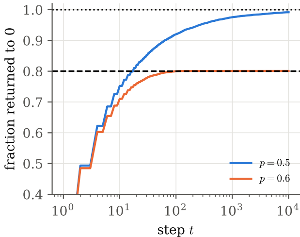
(b) symmetric walkers all come home
