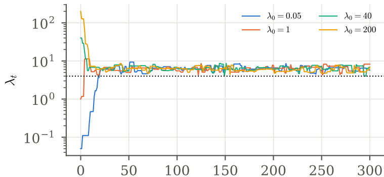
(a) N = 3 counts, prior B: first 300 steps
