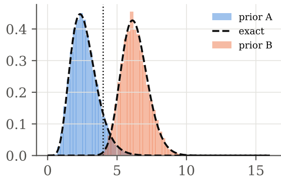
(c) posteriors, N = 3
