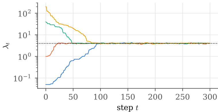
(b) N = 300 counts, prior B: first 300 steps
