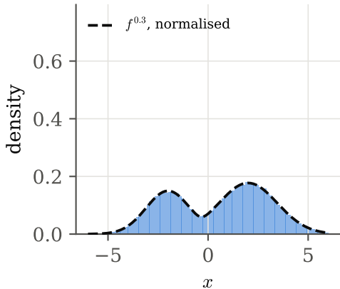
accept with \min(1, R^{0.3})
