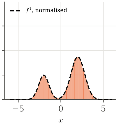
accept with \min(1, R^1)
