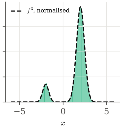
accept with \min(1, R^3)
