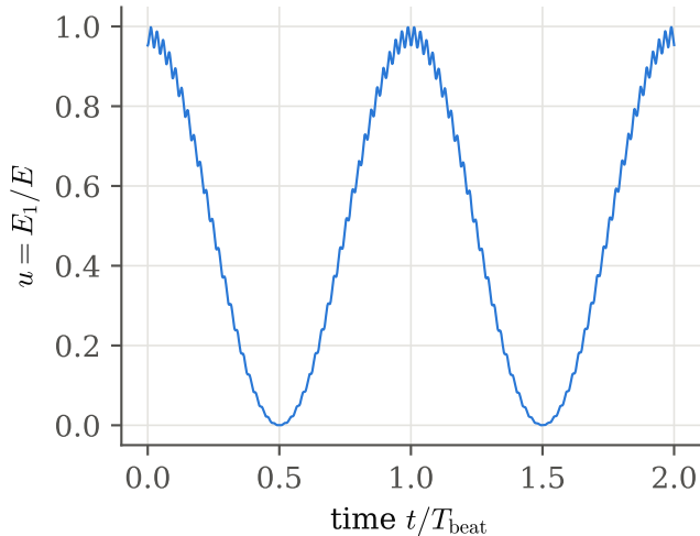
(a) the energy sloshes back and forth
