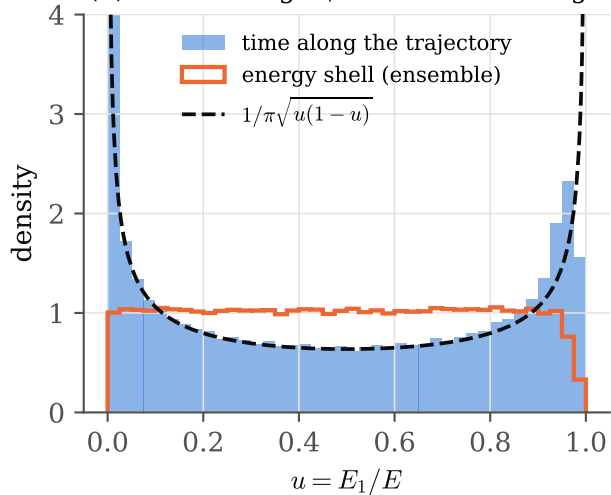
(b) time average \neq ensemble average
