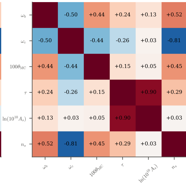
Planck 2018 TT+lowE chains
