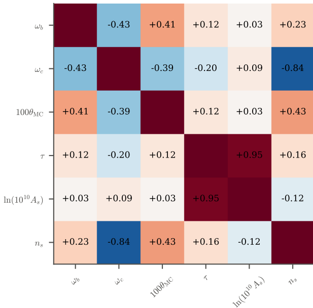
Fisher, Planck-like TT + \tau prior
