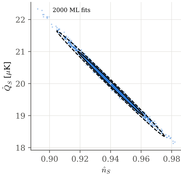
20' beam, w^{-1/2} = 15 \mu\text{K deg} : fits and Fisher
