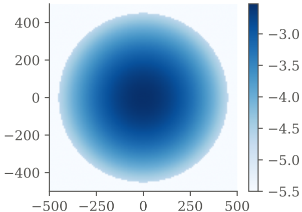
slice of \log_{10} \bar{n}(\mathbf{x})
