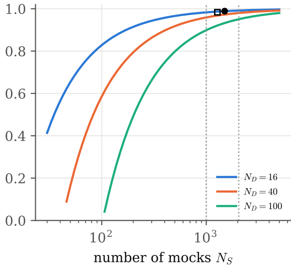
Hartlap factor
