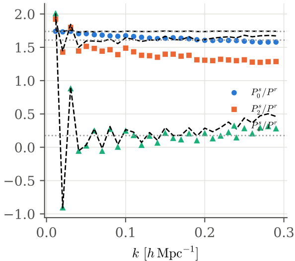
multipole / real-space power
