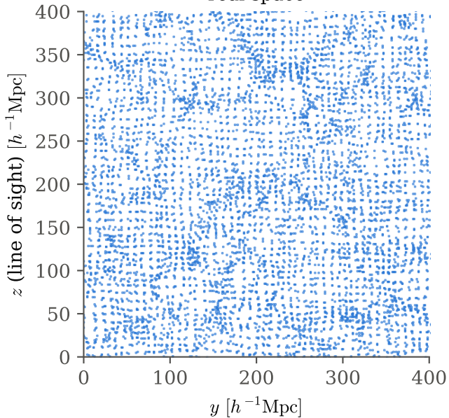
real space
