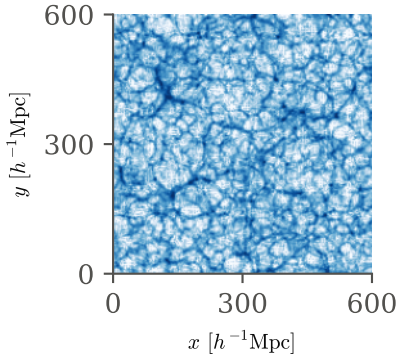
Zel'dovich universe
