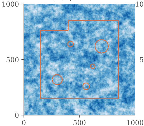
field \ln(1 + \delta) and the window
