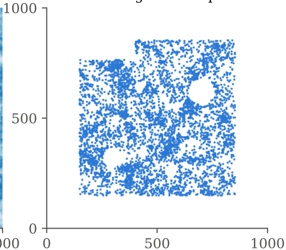
one catalogue: 4893 points
