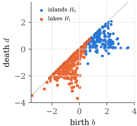
persistence diagram
