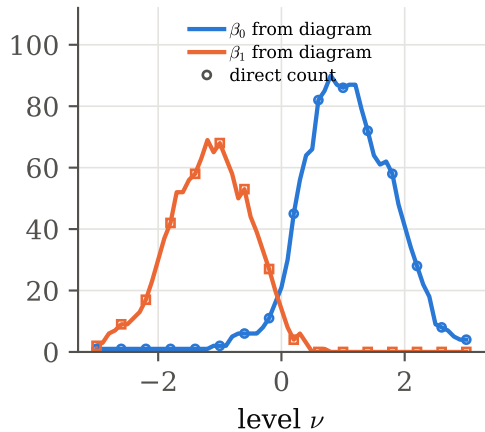
Betti curves
