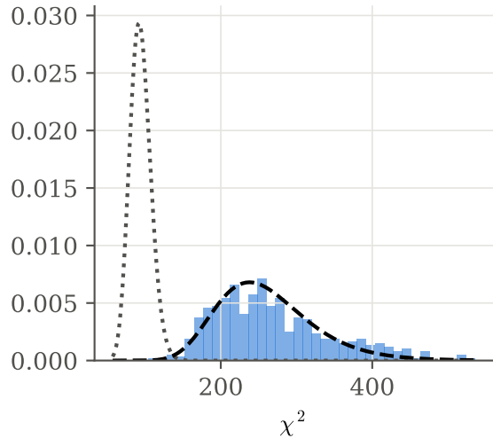
persistence hist., p = 94 , n = 150
