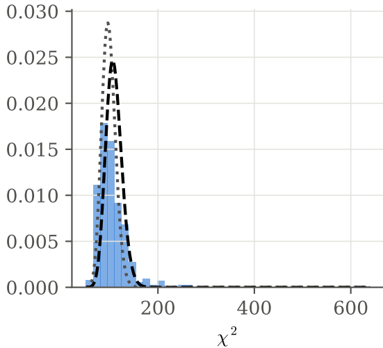
persistence hist., p = 98 , n = 1000
