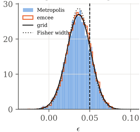
posterior, one map
