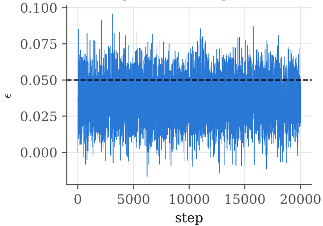
Metropolis chain, acceptance 0.59
