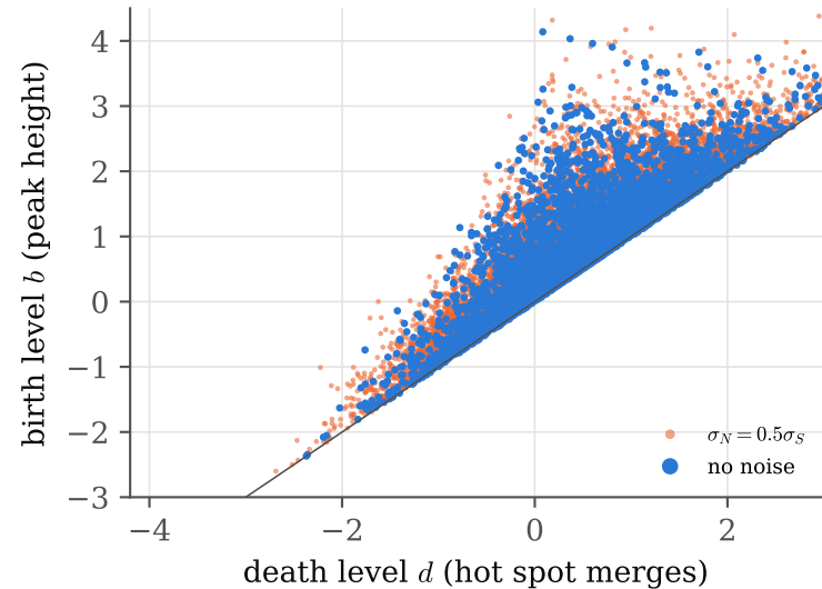
hot-spot diagram of one sky
