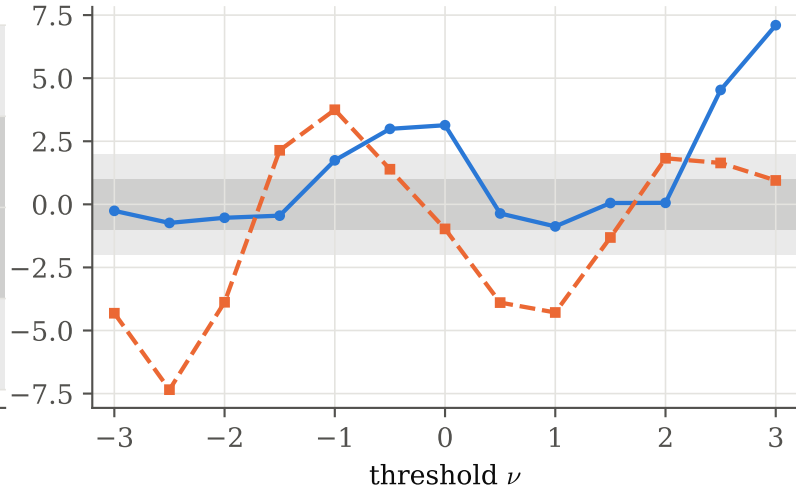
local-type sky, a = 0.15
